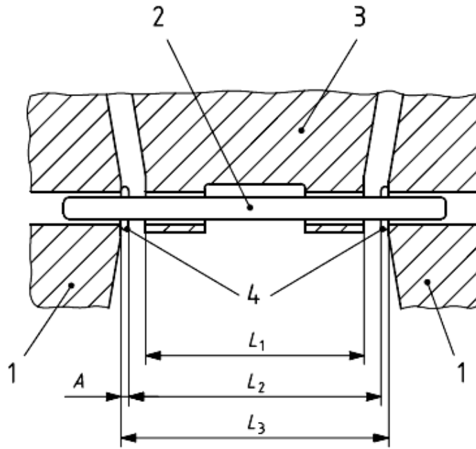
c) Total axial clearance, C_{TA}
