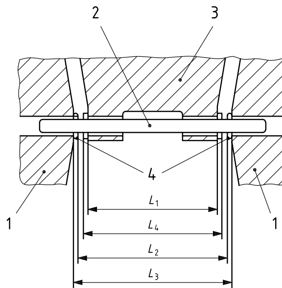
d) Inside bushing dimensions
